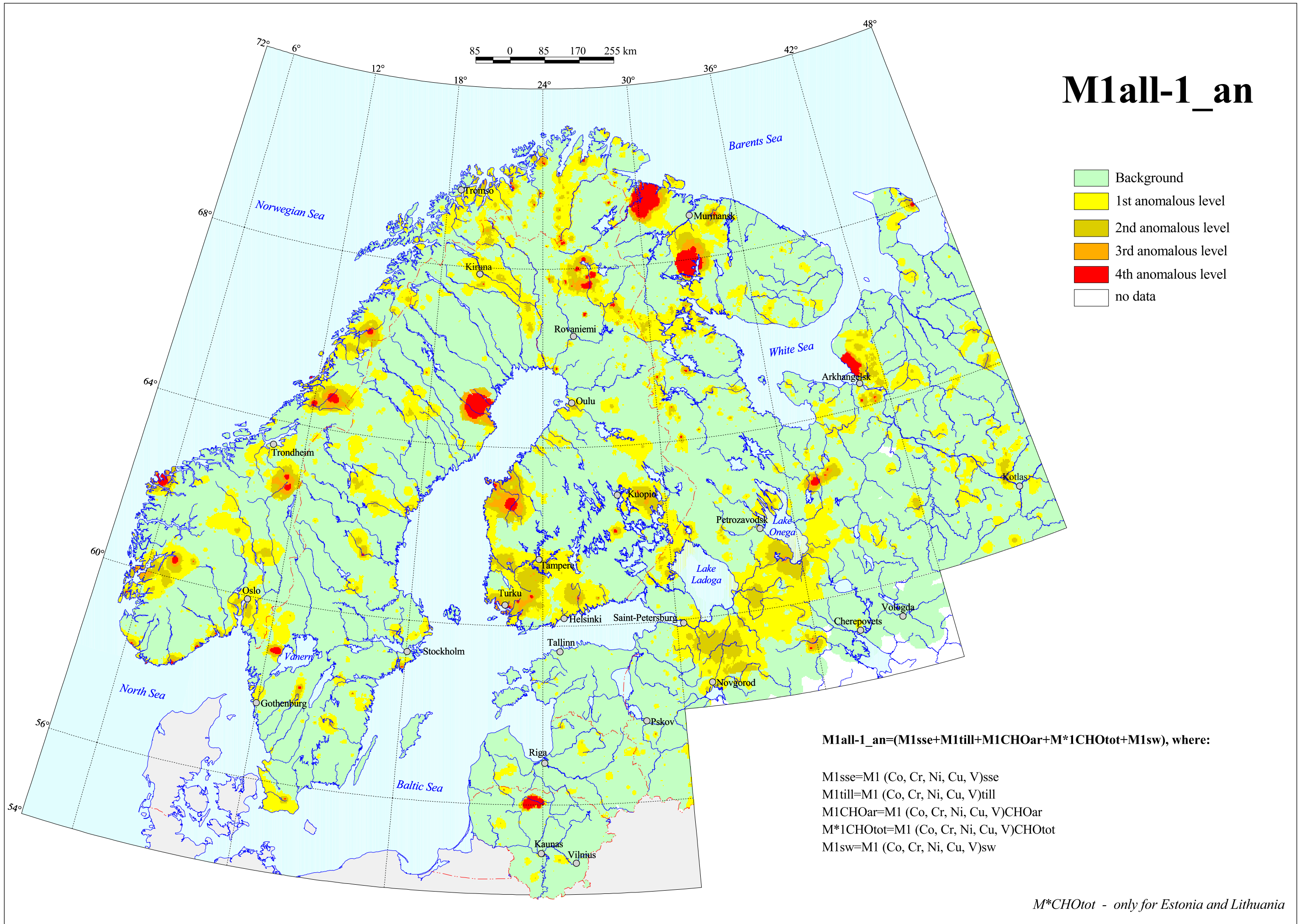
Integrated Anomalous Geochemical Fields, M1all-1_an
